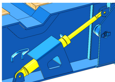
Cylinder For SR+ (2ea/box)
